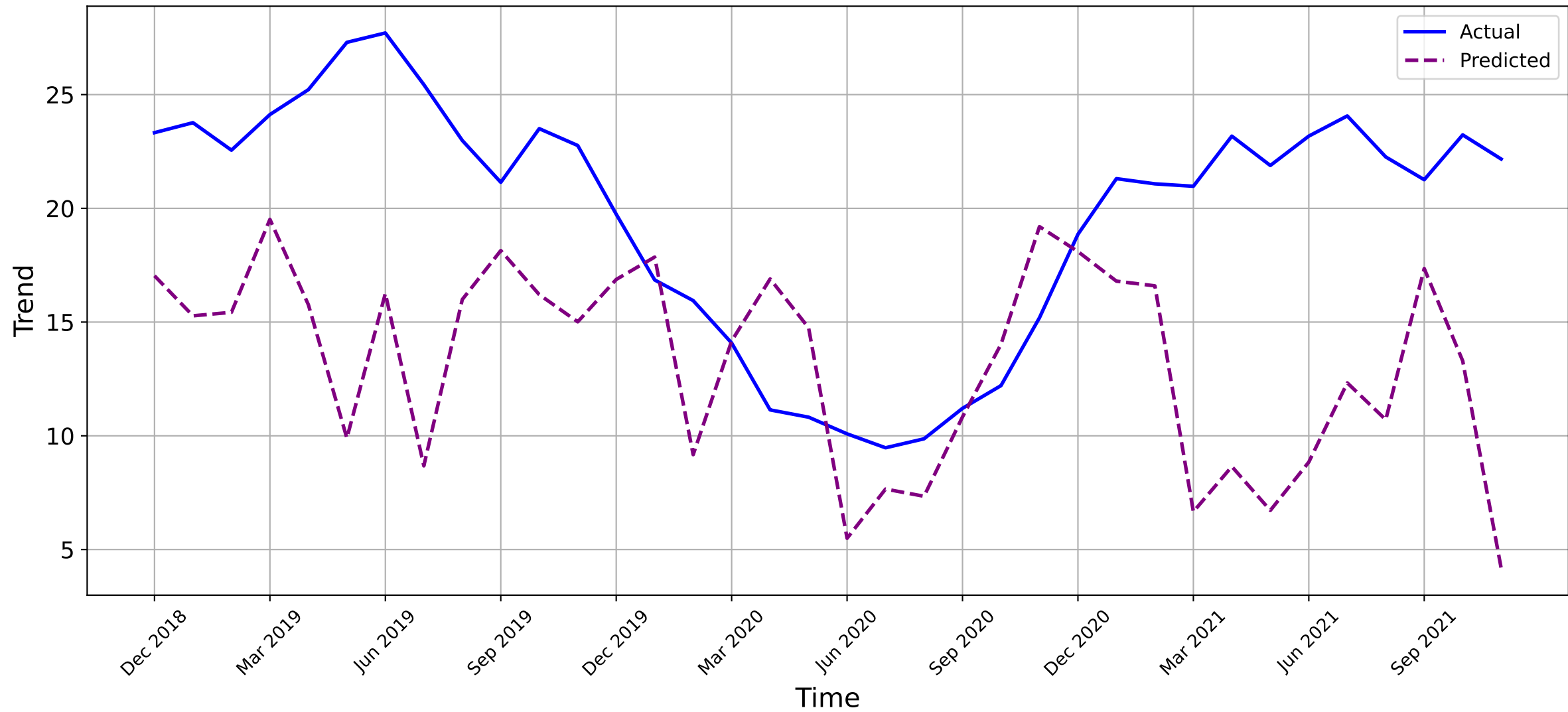
Solution_VPN_Mentions - Validation
